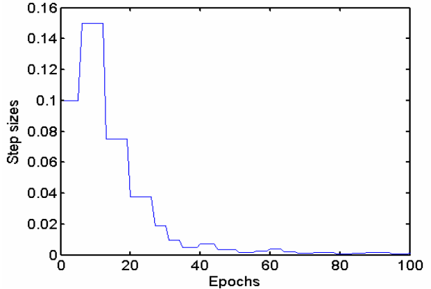
Fig. 7: Adaptation of parameter steps of ANFIS
