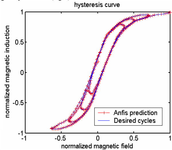
Fig. 8 : Hysteresis curves
