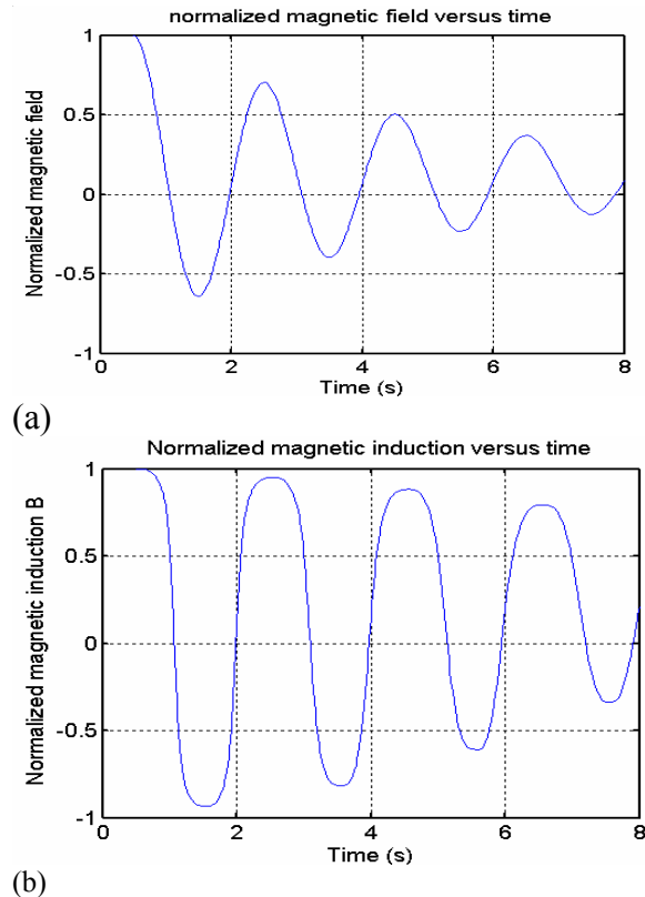
Fig.3: a- Normalized magnetic field and magnetic versus time b- Normalized magnetic induction versus time
