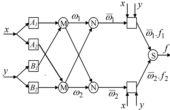
Fig. 1: ANFIS architecture
