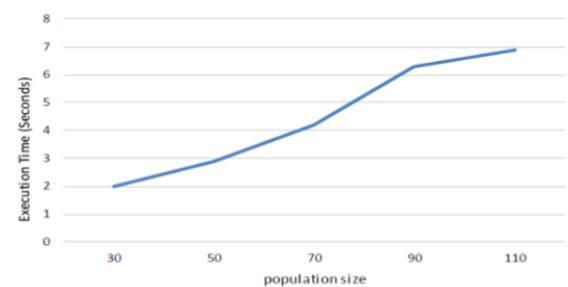
Fig. 18: Execution Time for Login information by Bryian Tan web Application
