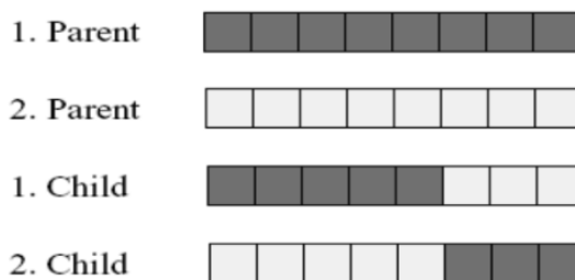
Fig. 2: Single Crossover at k = 5
