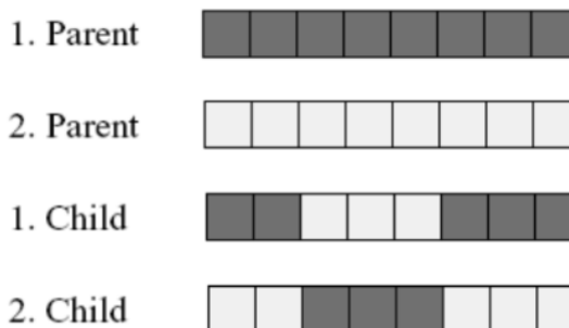
Fig. 3: Multi-point Crossover at k = 2 and k = 5
