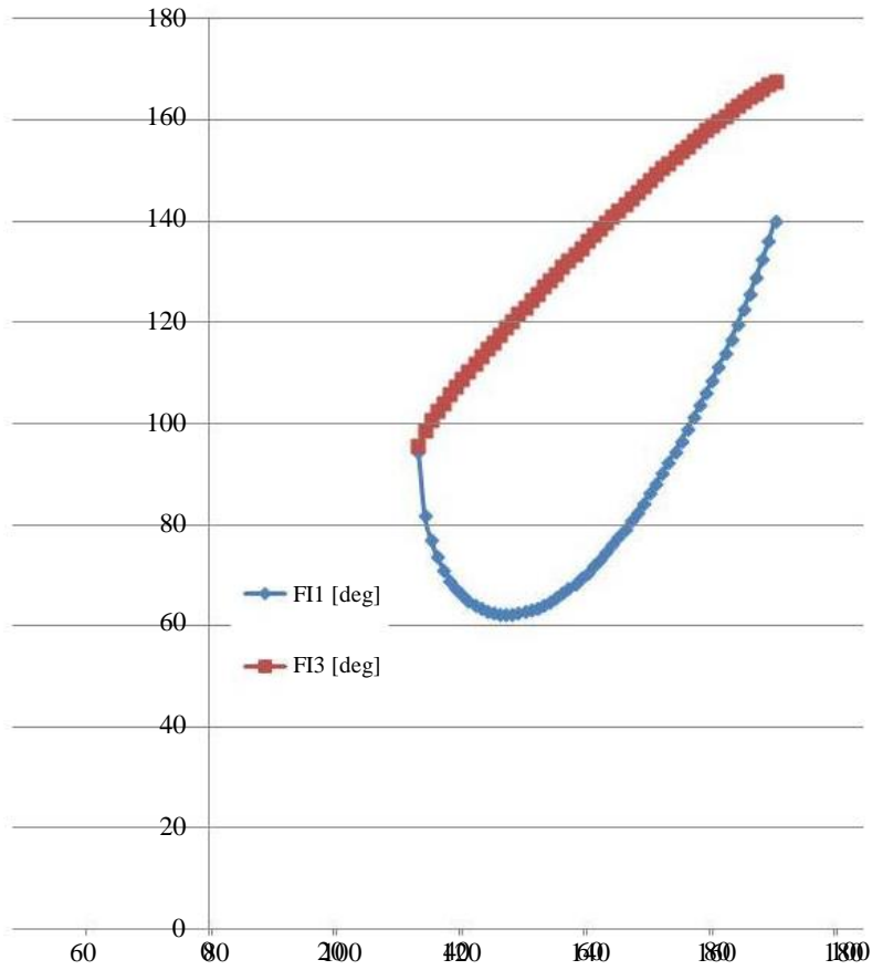
Fig. 7: Output values of the angles FI1 and FI3, depending on the value imposed at the input of the angle FI2 on the abscissa, for version I
