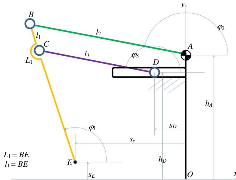
Fig. 5: Kinematic diagram of the planar mechanism 2R from the component of the 3R space manipulator
